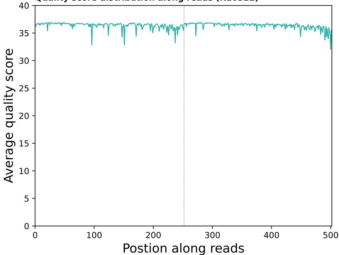
Quality score distribution along reads (R10522)
